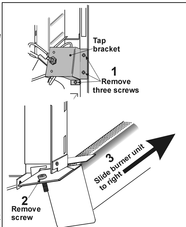
Figure 16. Burner module removal
