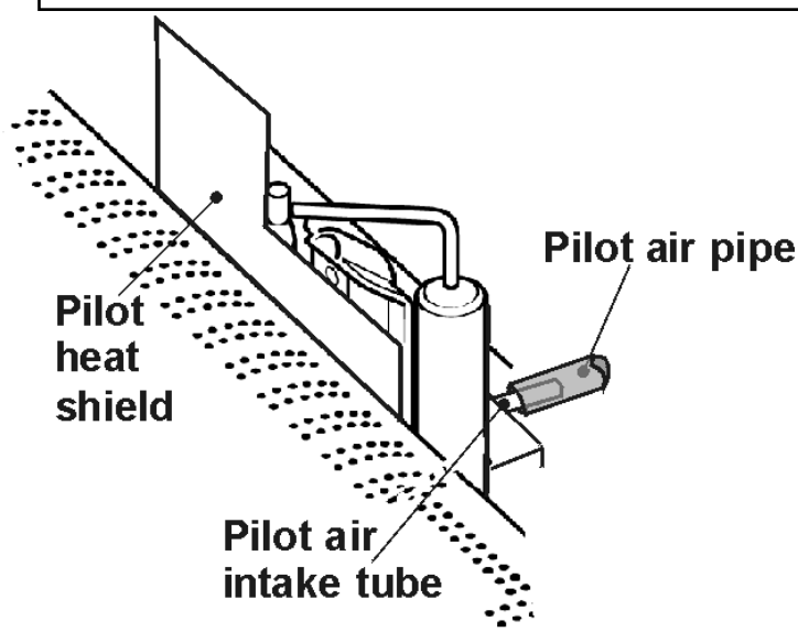
Figure 17. Pilot air pipe location
