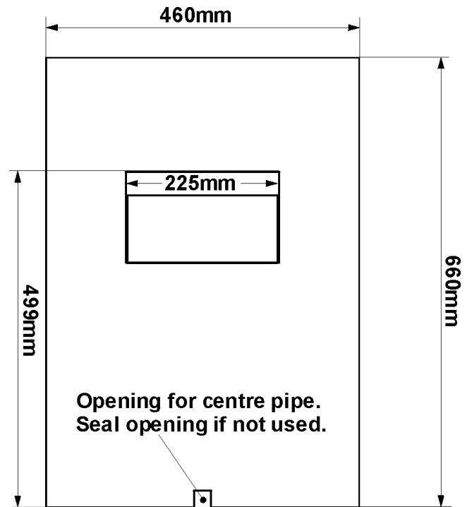
Figure 9. Closure plate.
