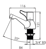
Bath Tap Pair with Lever UNEXTPBTHLE
