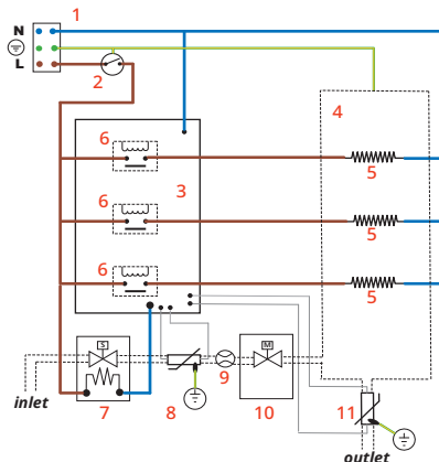
Fig.4 Tri-HUB Wiring Diagram
