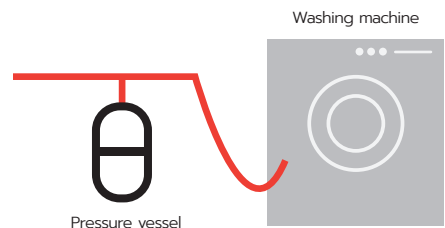
Figure 25: Water hammer protection
