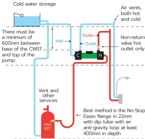
Figure 19: Anti-gravity loop (AGL)
