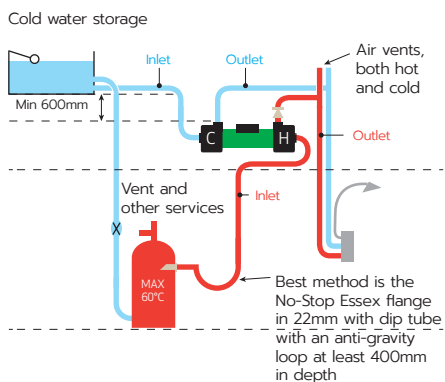
Figure 7: Typical Right Pump Installation - pump located above the cylinder
