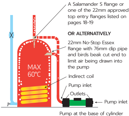
Figure 3: Hot water supply method
