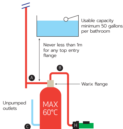
Figure 23: Warix flange
