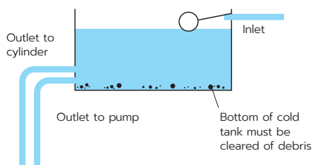
Figure 1: Tank inlet and outlet position
