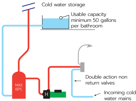
Figure 12: Tank fed (hot) with mains cold
