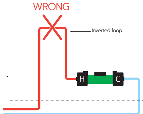
Figure 24: Inverted loops
