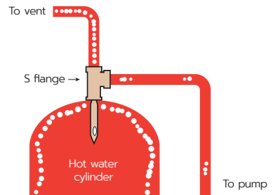
Figure 22: S flange
