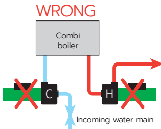
Figure 20: Combi boilers
