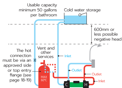
Figure 6: Typical Right Pump Installation - pump located at base of the cylinder
