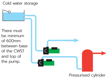
Figure 11: Pressurised cylinder or Combination boiler system
