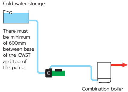
Figure 13: Typical combi boiler system
