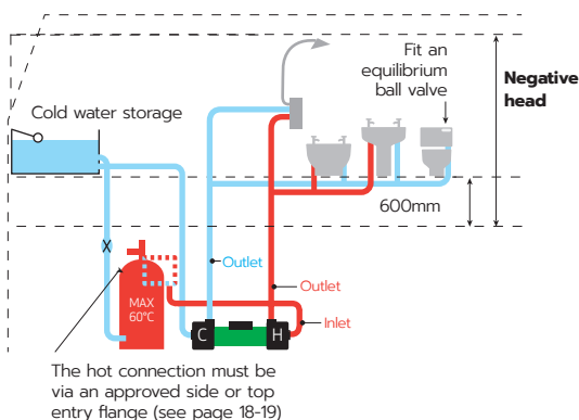
Figure 8: Negative head
