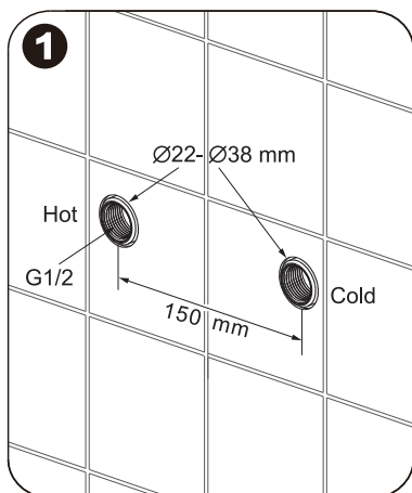
1. Inlet pipework should be at 150mm pipe centers.
