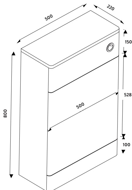
Dimensions (measurements in mm)
