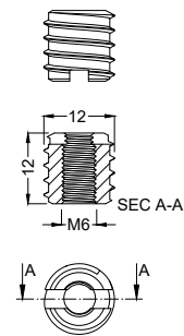
BUSHING DETAIL
