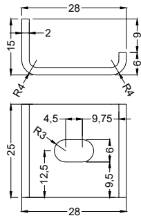
HOOK DETAIL
