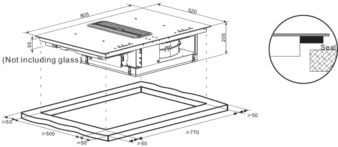
Hole size of cabinet: 765x495mm
