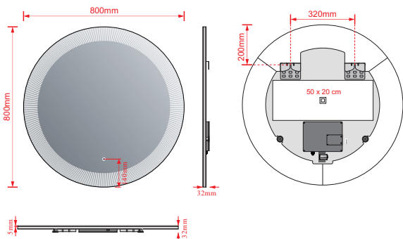
94.0012 DL-73C-80 Size: Ø800mm
