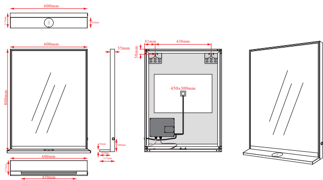
94.0002 DL-03BL-P-6080MB Size: 600x800mm
