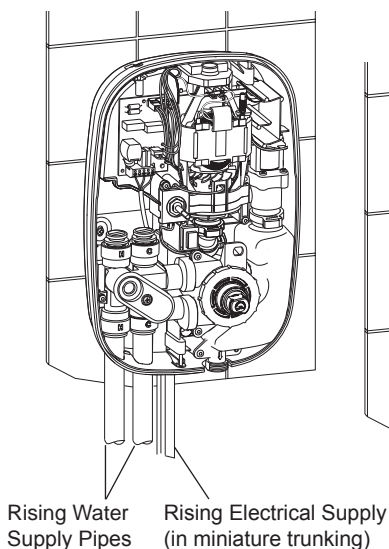
Bottom Entry Supply Configuration
