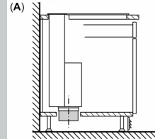
A: Exterior wall – U-value ≤ 0.5 W/(m²K)
