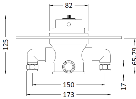
CONCEALED VALVE
