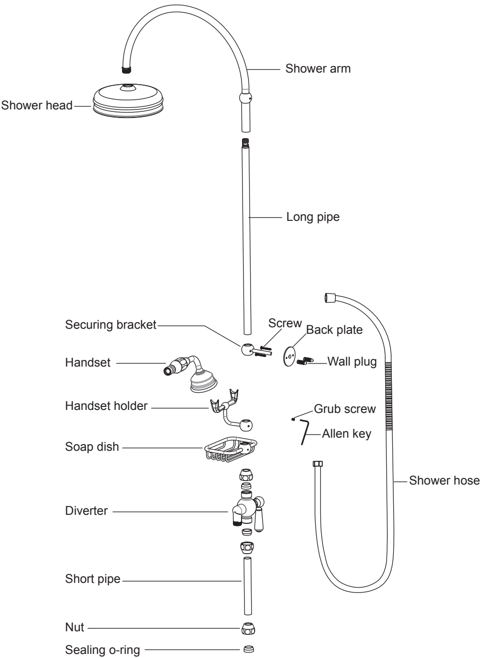
Exploded Diagram
