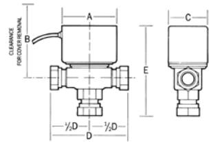
Dimensions (mm)
