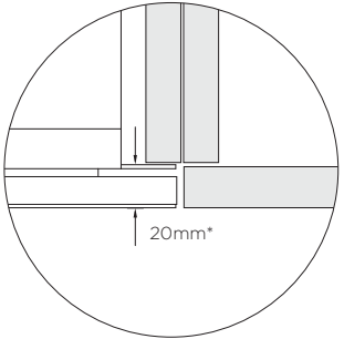
FLUSH INSTALL
