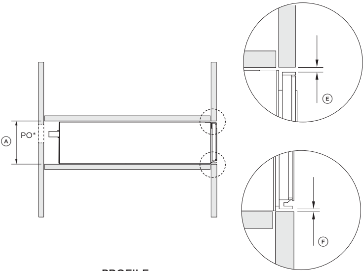
PROFILE
