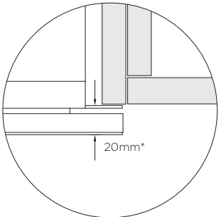
PROUD INSTALL
