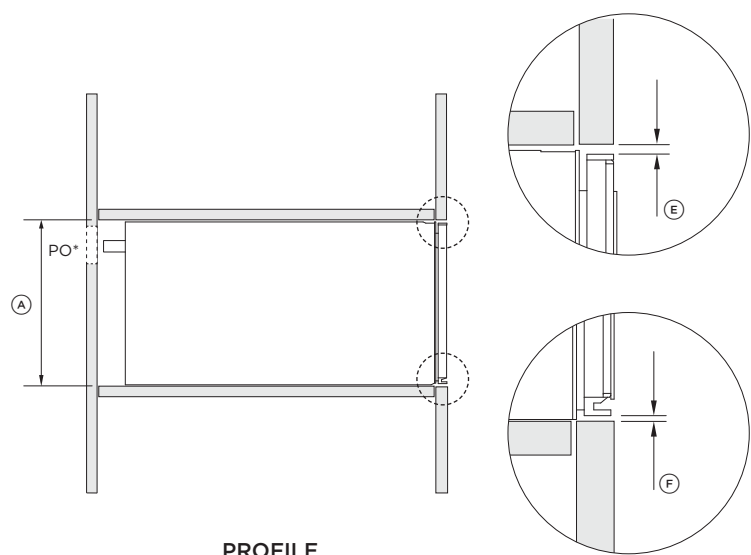
PROFILE
