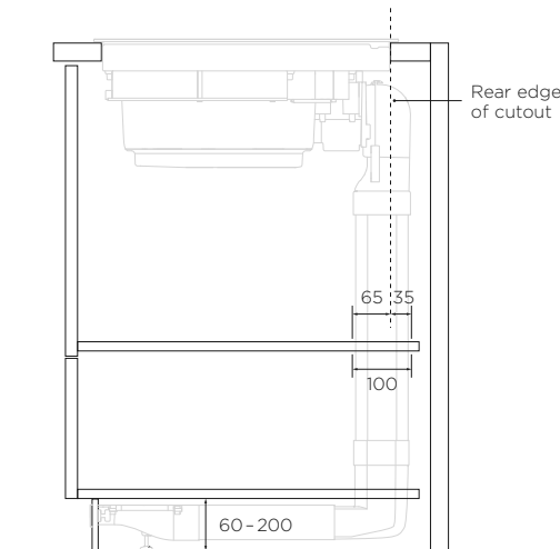
PROFILE: SHELVING
