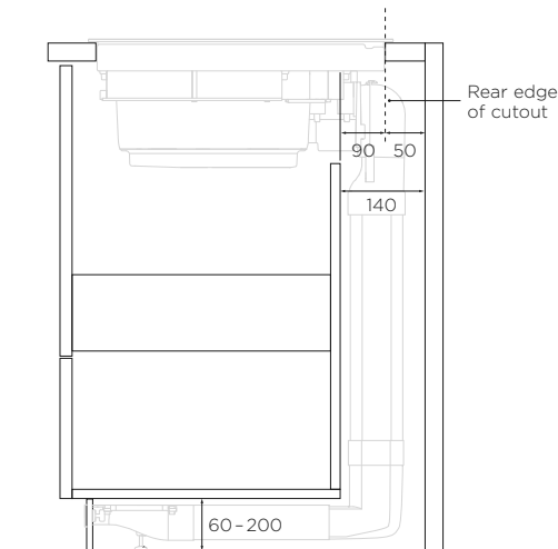
PROFILE: SEPARATE HOUSING
