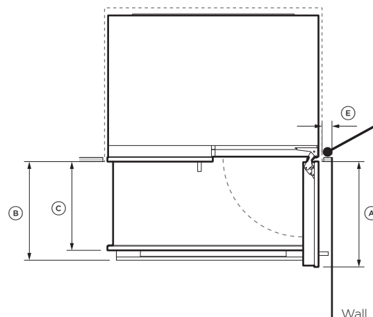
90° DOOR OPENING
