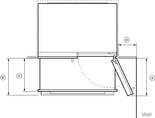
115° DOOR OPENING (FULL INTERNAL ACCESS)
