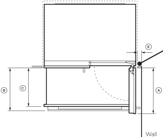
90° DOOR OPENING
