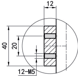
B SECTION
