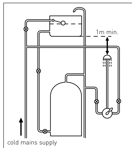
Gravity Fed Hot and Mains Cold
