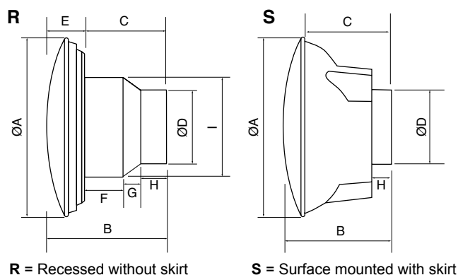
R = Recessed without skirt
