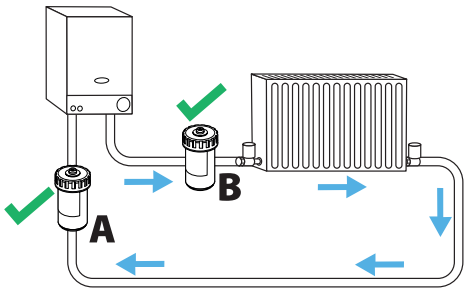
Combi/Sealed system
