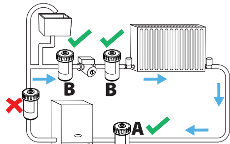
Open vented system
