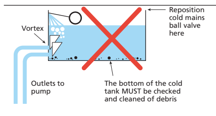
Figure 20: Aeration
