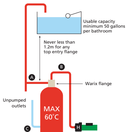
Figure 30: Approved flanges
