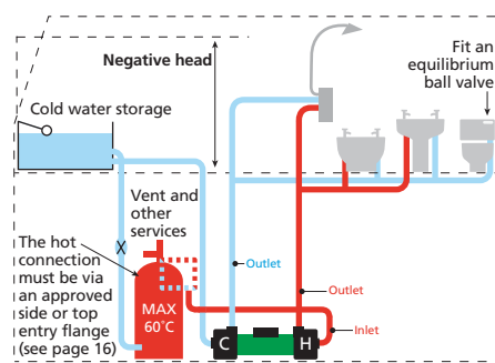
Figure 10: Negative head
