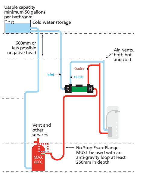
Figure 13: Instantaneous electric showers and
