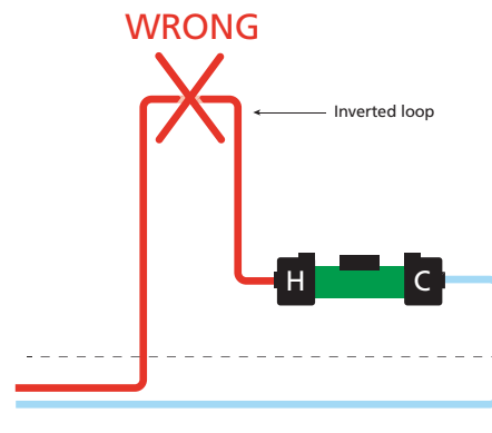
Figure 31: Inverted loops
