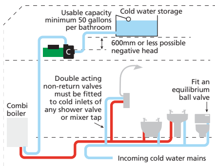
Figure 14: Pressurised cylinder or Combination boiler system
