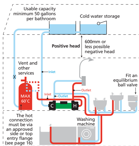
Figure 11: Positive head
