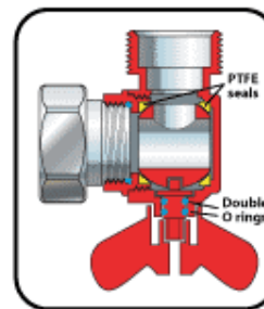
Inlet/Outlet valve X-section
