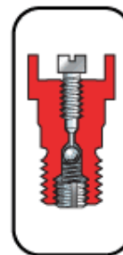
Bleed Valve X-section
